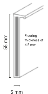
D 60 (without sealing lip)
